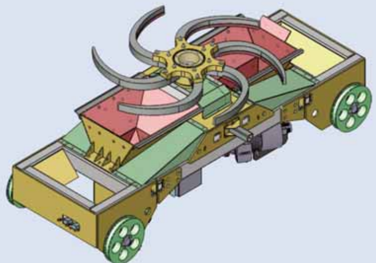
EF Rotary discharge extractor
