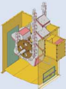
ESPLV - BUCKET ELEVATOR with double lateral chains (for large capacity)
